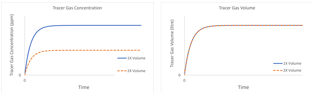
Figure 6 Two offices of different volumes ventilated with the same constant air change rate: (left) concentration of tracer gas in the space; and (right) volume of tracer gas in the space
