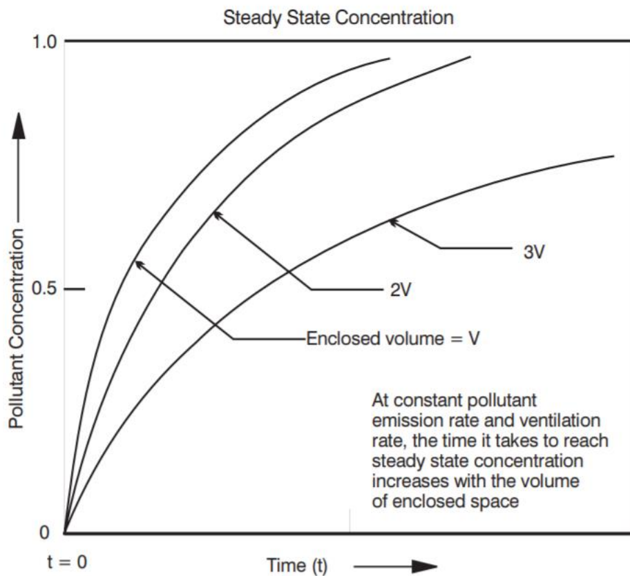
Figure 7 The building as a fresh air reservoir (reproduced with permission from A Guide to Energy Efficient Ventilation (Liddament, 1996))
