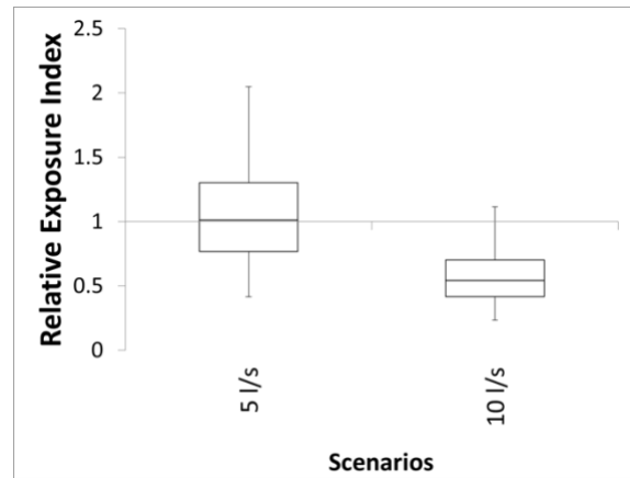
Figure 9a (left) A sample calculation using ventilation rates of 5 l/s/p and 10 l/s/p with no air cleaner; and Figure 9b (right) the resulting box whisker plot
