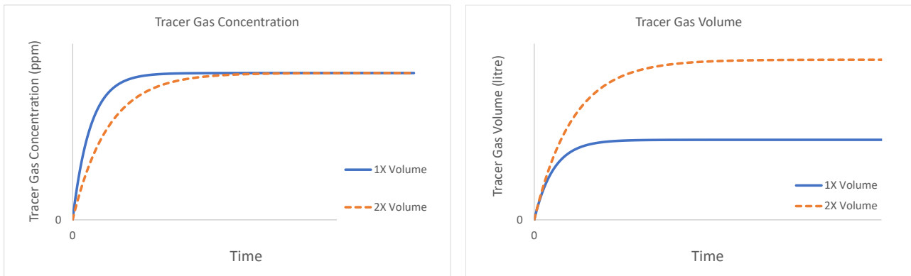
Figure 5 Two offices of different volumes ventilated with the same constant volume flow rate: (left) concentration of tracer gas in the space; and (right) volume of tracer gas in the space
